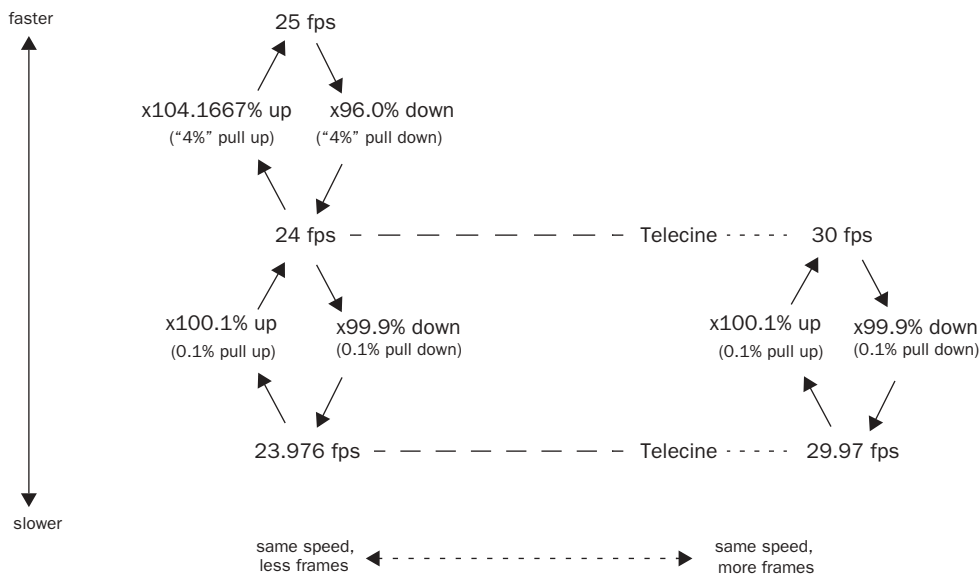
Figure 44. Frame rates, telecine transfers, and relative playback speeds
