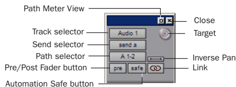
Send window standard controls, Windows (left) and Macintosh (right)
