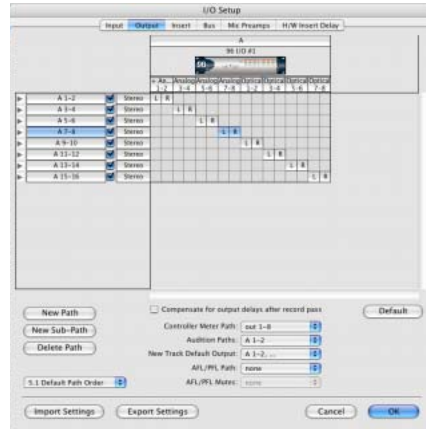
I/O Setup dialog Output paths (Pro Tools HD)
