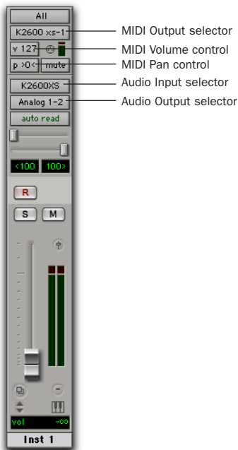
Instrument track configured to control and monitor an external MIDI instrument (K2600XS)
