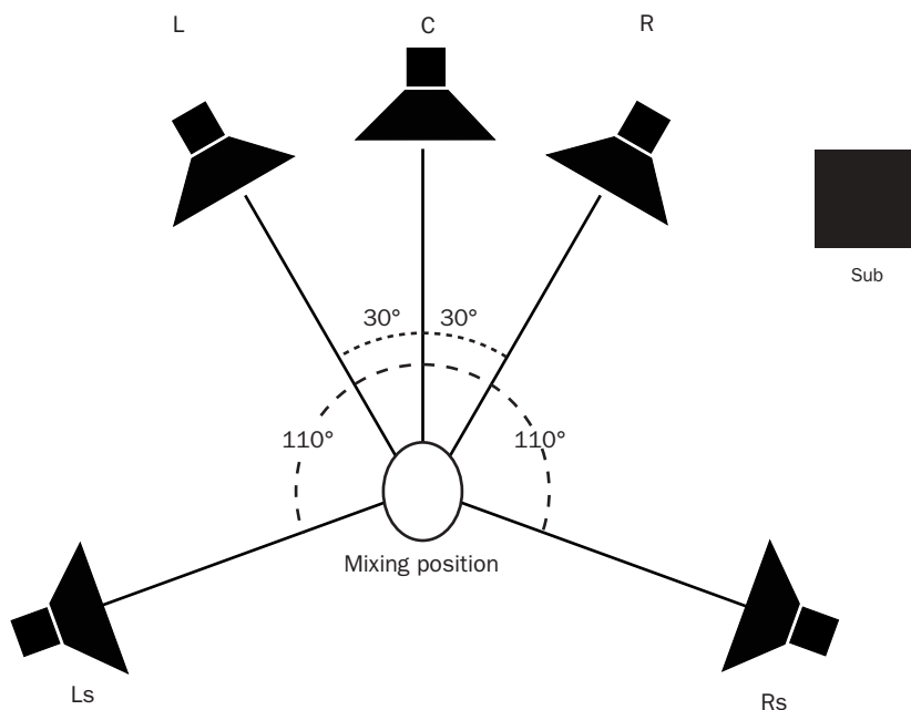
Figure 31. Example of speaker arrangement for 5.1 mixing and monitoring (SMPTE specification). Sub placement is variable, while all other speakers should be as close to the suggested angles as possible.
