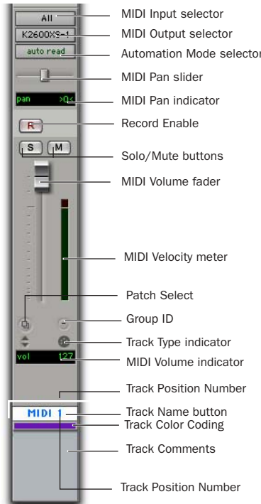
MIDI channel strip
