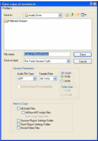
Save Copy In dialog
